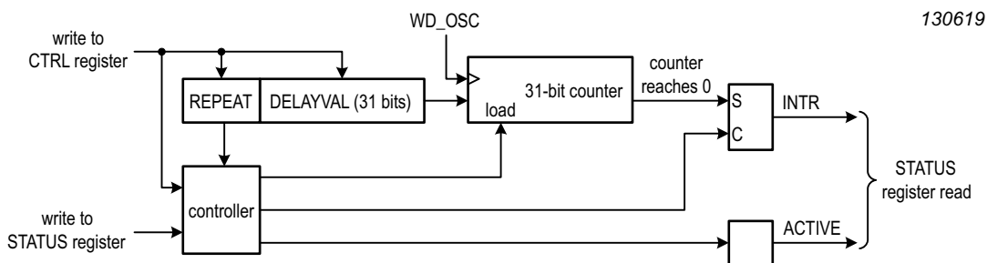
Fig 44. Micro-Tick Timer block diagram
