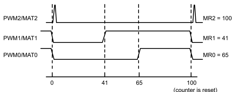
Fig 34. Sample PWM waveforms with a PWM cycle length of 100 (selected by MR3) and MAT3:0 enabled as PWM outputs by the PWCON register.
