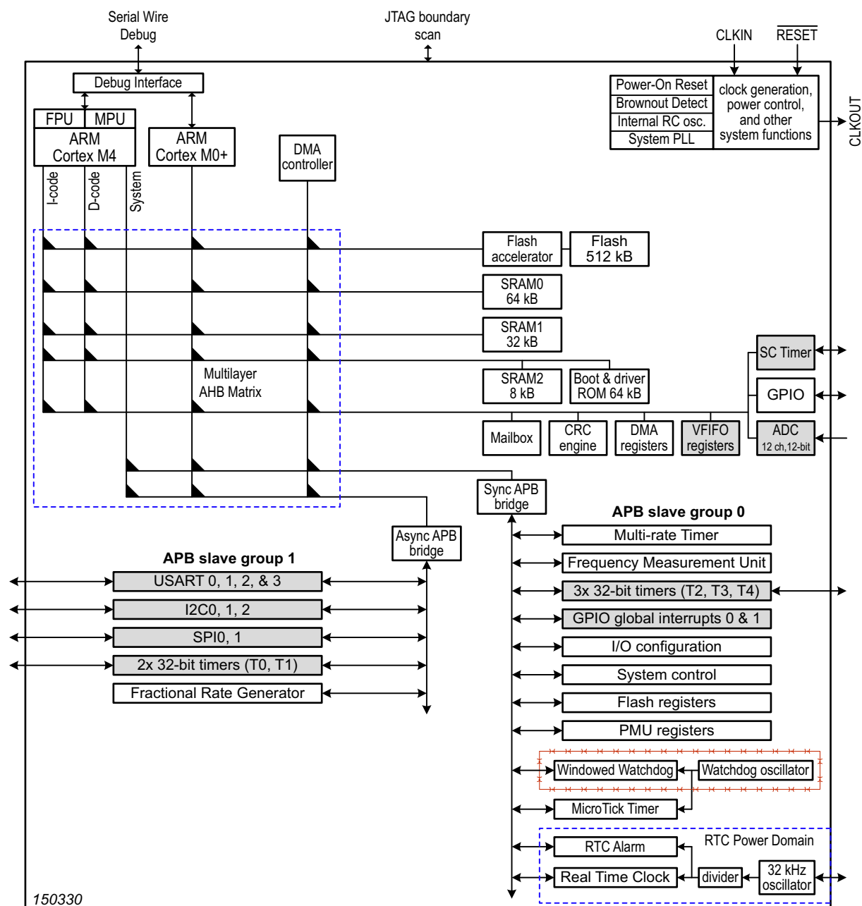
Fig 1. Block diagram
