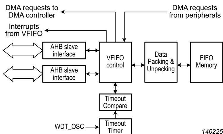
Fig 55. System FIFO conceptual block diagram
