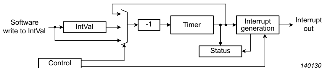
Fig 41. MRT block diagram
