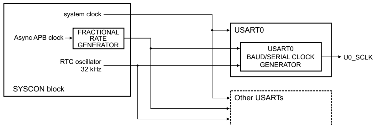
Fig 45. USART clocking
