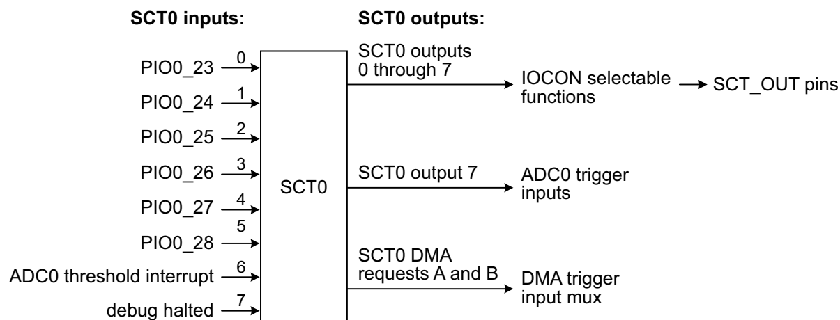
Fig 21. SCT connections
