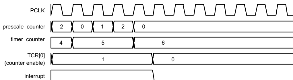
Fig 33. A timer cycle in which PR=2, MRx=6, and both interrupt and stop on match are enabled
