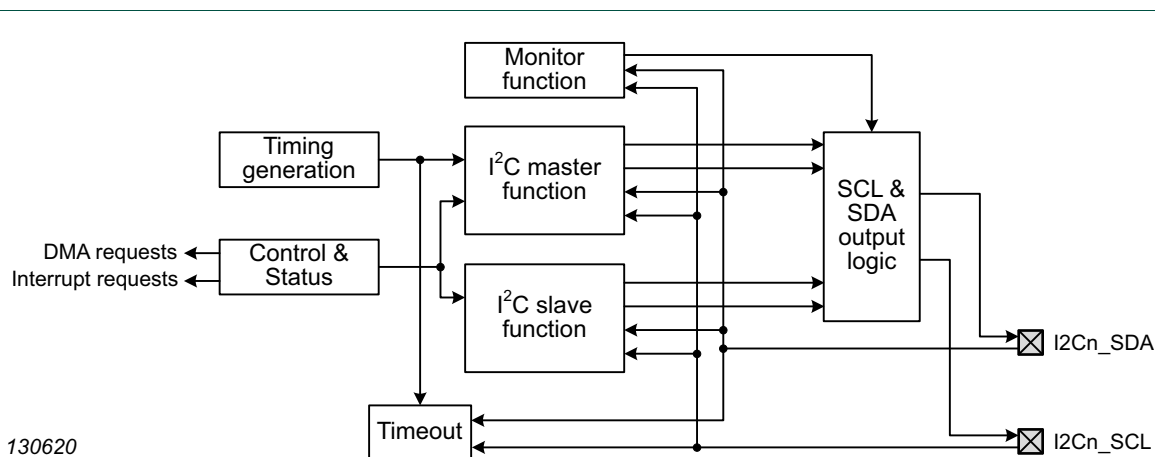
Fig 54. I 2 C block diagram
