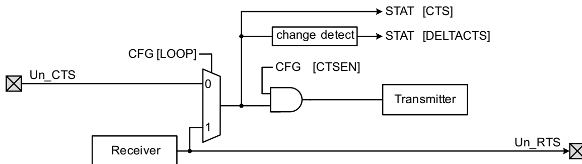
Fig 47. Hardware flow control using RTS and CTS
