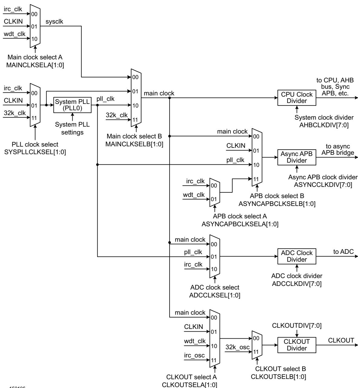
Fig 5. Clock generation
