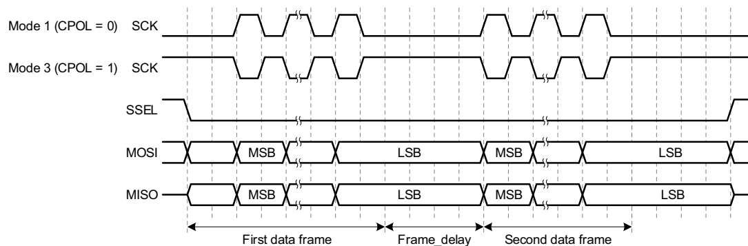
Fig 51. Frame_delay
