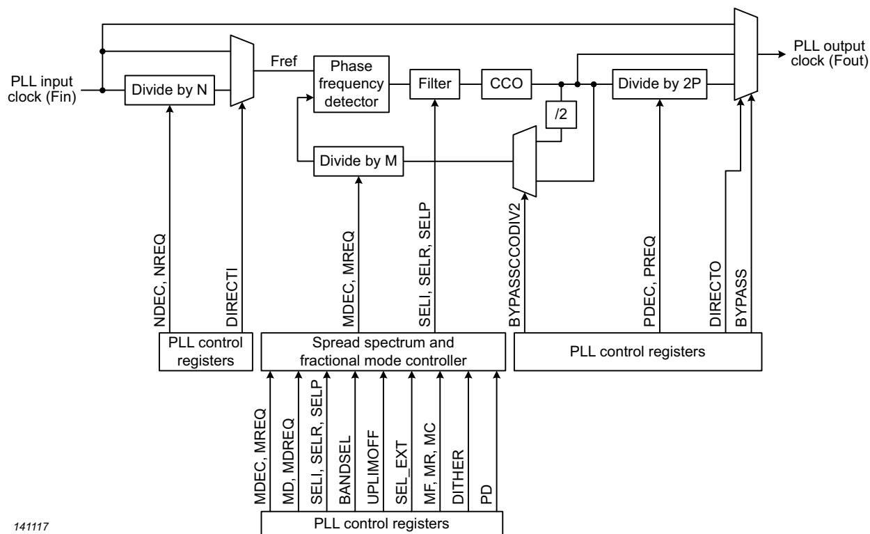
Fig 8. PLL block diagram showing spread spectrum and fractional divide operation
