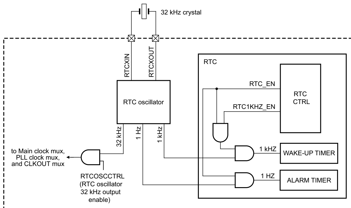
Fig 40. RTC clocking
