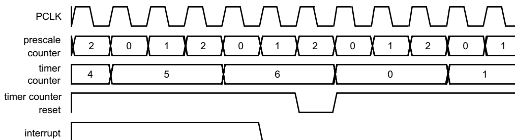
Fig 32. A timer cycle in which PR=2, MRx=6, and both interrupt and reset on match are enabled
