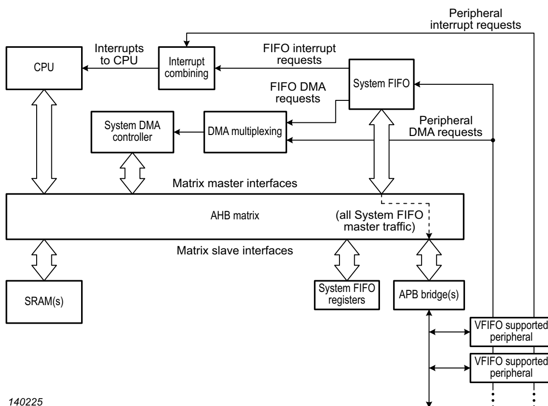
Fig 56. FIFO system
